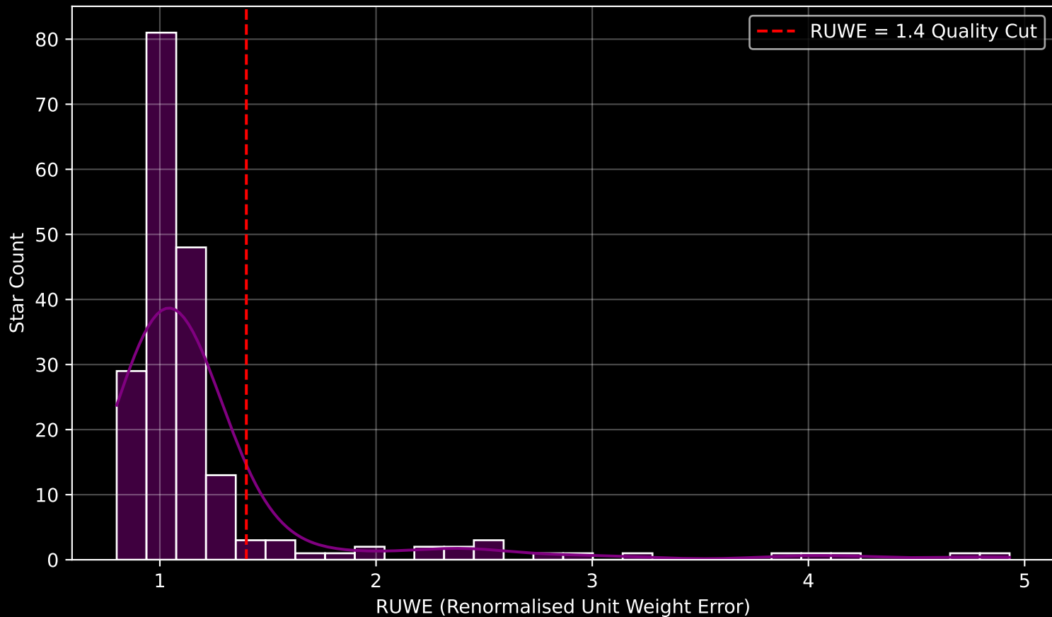
GAPOGEE DR17 Field [178+28_MGA] RUWE Distribution (n= 196)
