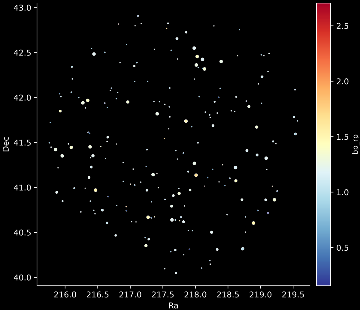
APOGEE DR17 Field: [178+28_MGA] Stars: 202
