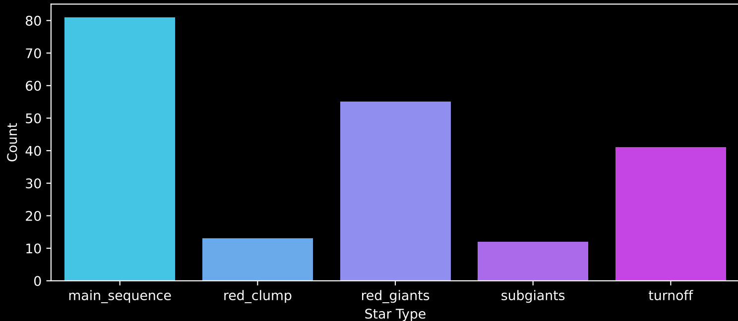
APOGEE DR17 Field: [178+28_MGA] Count plot of Star Type
