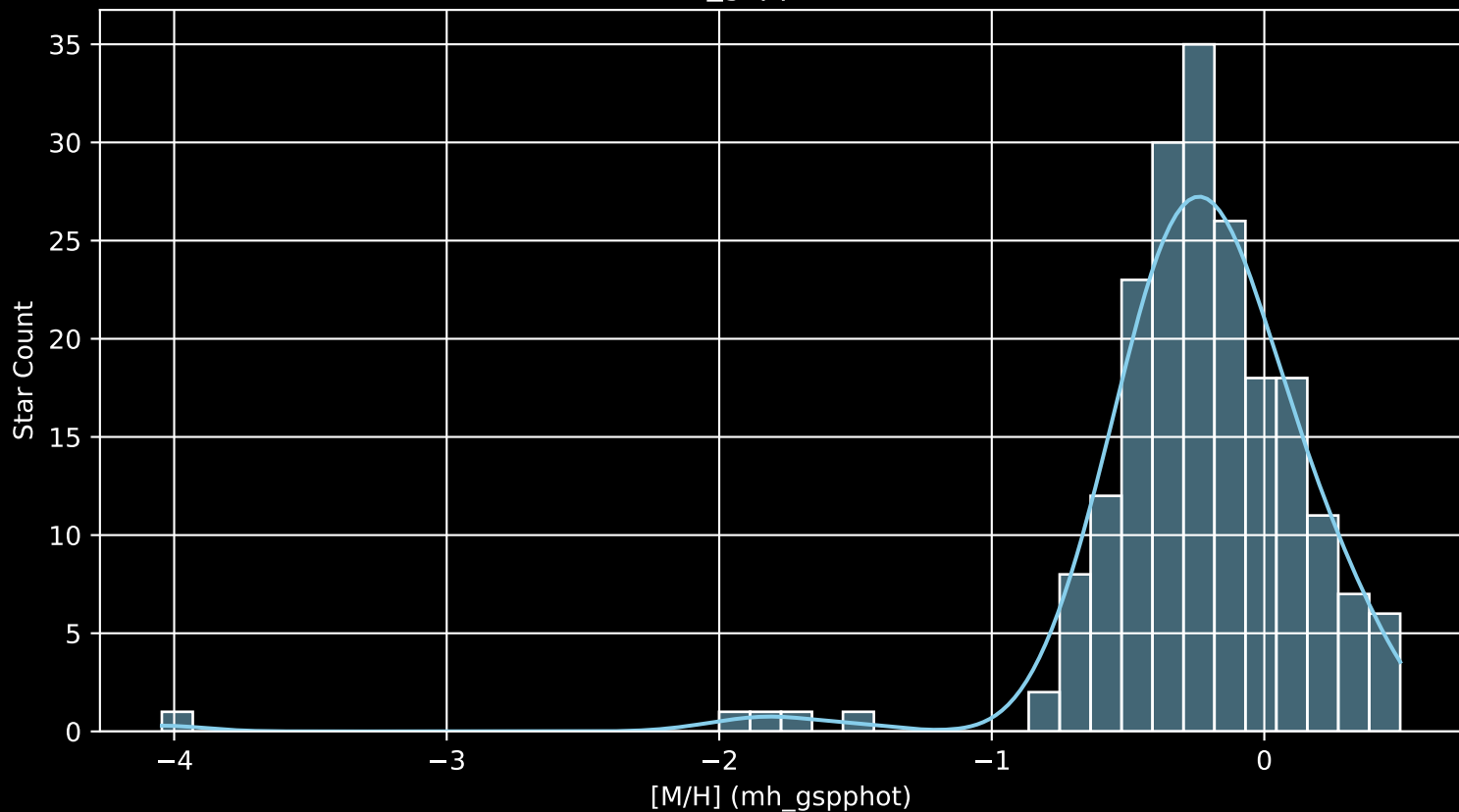
APOGEE DR17 Field: [178+28_MGA [M/H] (mh_gspphot) (n= 201)
