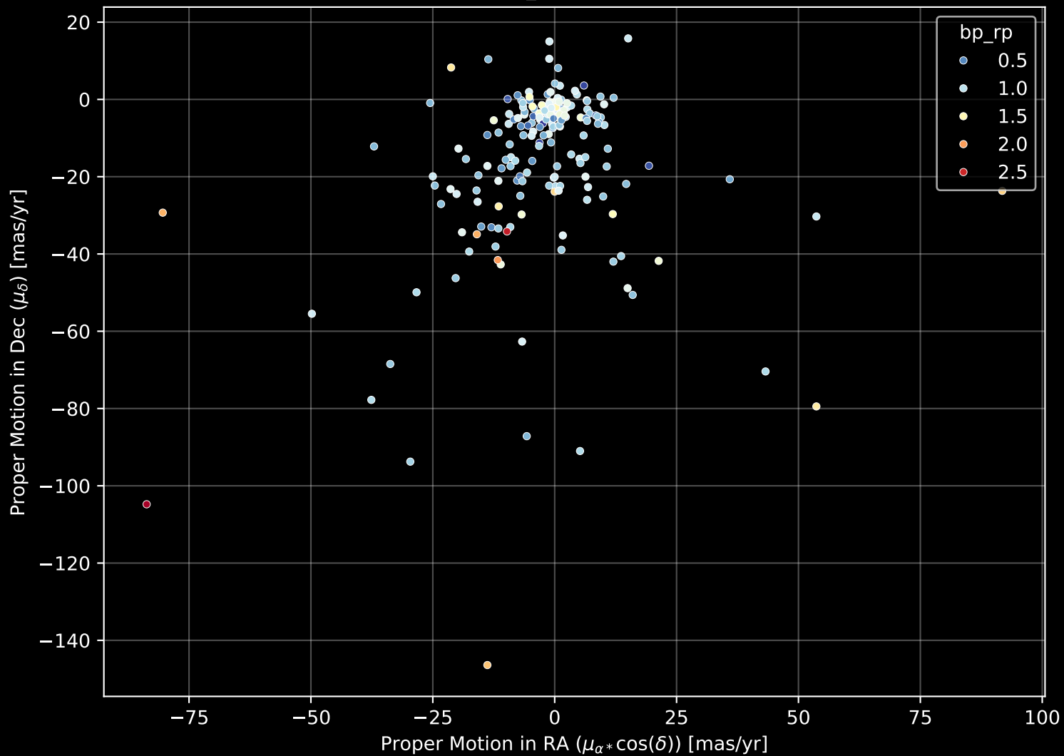
APOGEE DR17 Field: [178+28_MGA] Proper Motion Diagram (n= 202)
