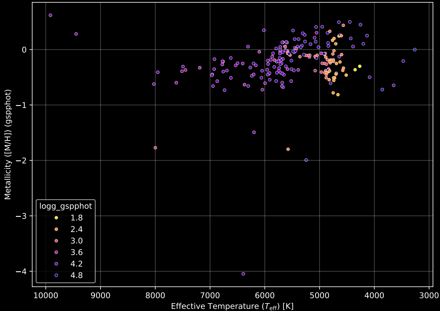
APOGEE DR17 Field: [178+28_MGA] Stellar Population Parameters (n= 202)
