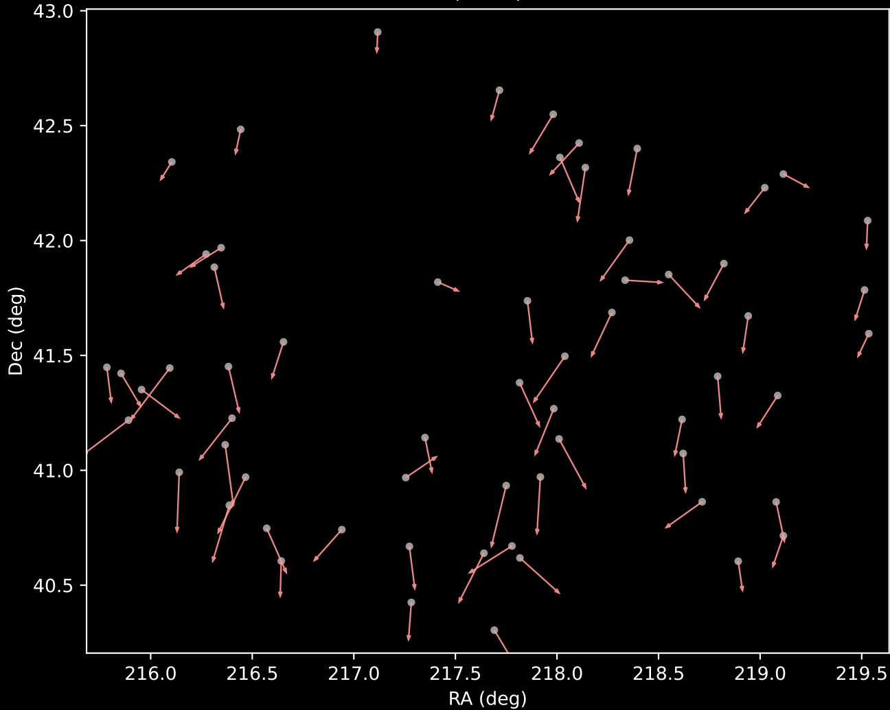
APOGEE DR17 Cluster 7 Proper Motion Vectors (n=62)
