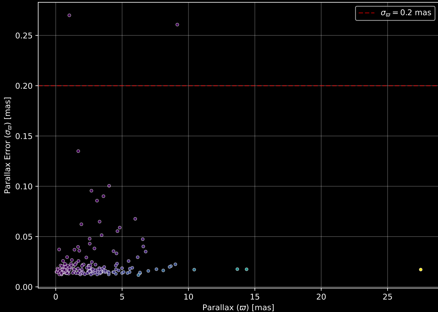
APOGEE DR17 Field: [178+28_MGA] Parallax Quality (n= 202)
